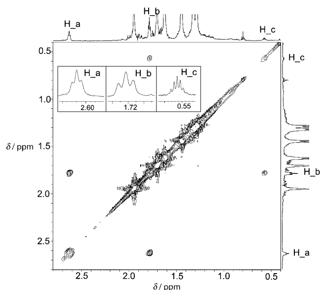
Figure 2. a) Part of the ^1\text{H} , ^1\text{H} -COSY spectrum of [(\text{para})_3\text{Mg}_8\text{H}_{10}] (500 MHz, [\text{D}_8]\text{toluene} , 25 °C). The insets show the signals for the three types of hydride ligands H a , H b , and H c ; ^2J(\text{H}_a, \text{H}_b) = 5.2 Hz and ^2J(\text{H}_b, \text{H}_c) = 4.5 Hz.
