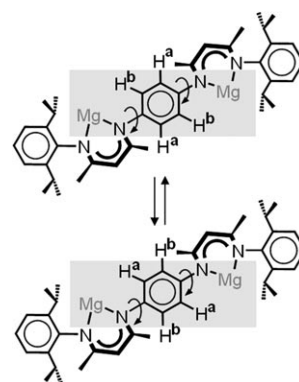
Scheme 2. Rotation of the para -phenylene bridge, which leads to coalescence of the H a and H b signals in the ^1\text{H} NMR spectrum at elevated temperature.
